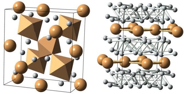
FIG. 1 (color online). Novel structures of silane. Large atoms depict Si, while small atoms represent H. Left : Fdd2 silane, stable between 25 and 55 GPa. Right : Pbcn silane, which is metallic, superconducting and favored above 220 GPa.
